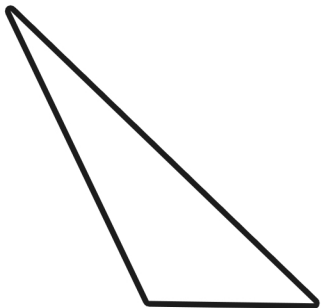
scalene triangle
