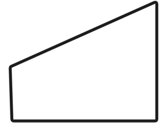
trapezoid
