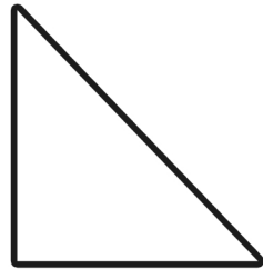
right-angled triangle
