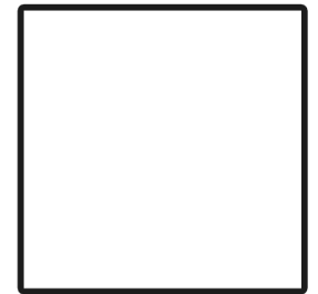
square
